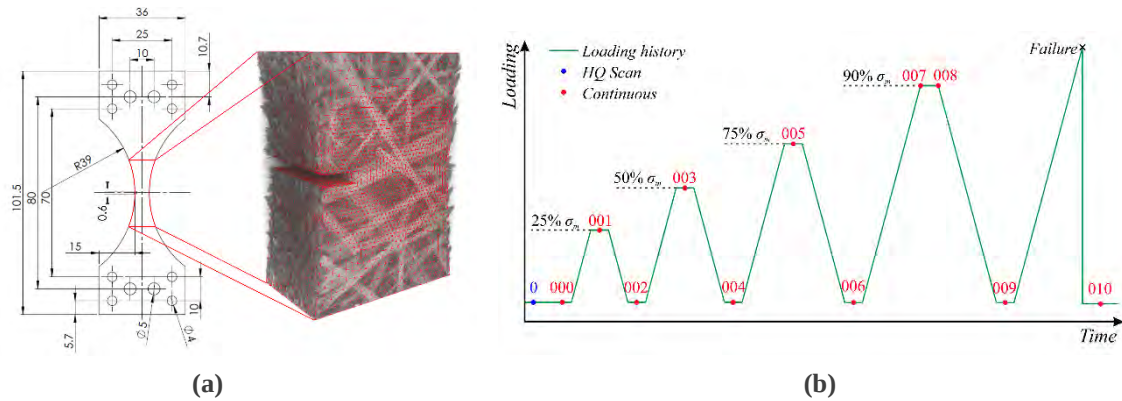
Figure 22. (a) Geometry of the dogbone specimen together with the studied ROI. (b) Schematic representation of the loading and acquisition history of the in-situ cyclic experiment.
