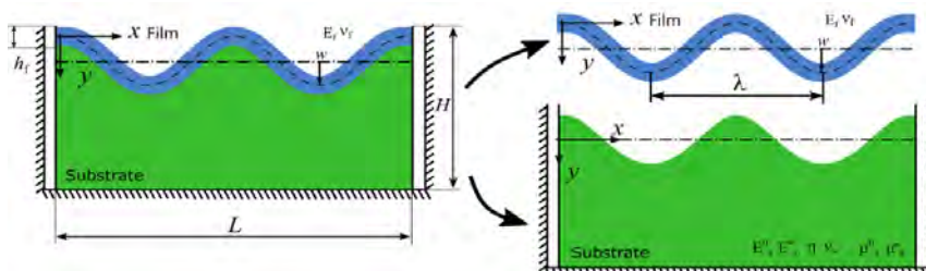
Figure 1. Elastic film and the viscoelastic substrate as separate structural elements.
