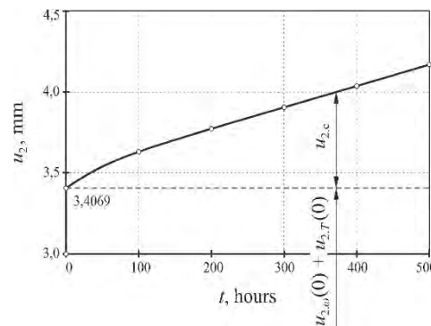
Figure 1. The dependence of the radial displacement, u_z , of the external boundary of the gas turbine disk on time t
