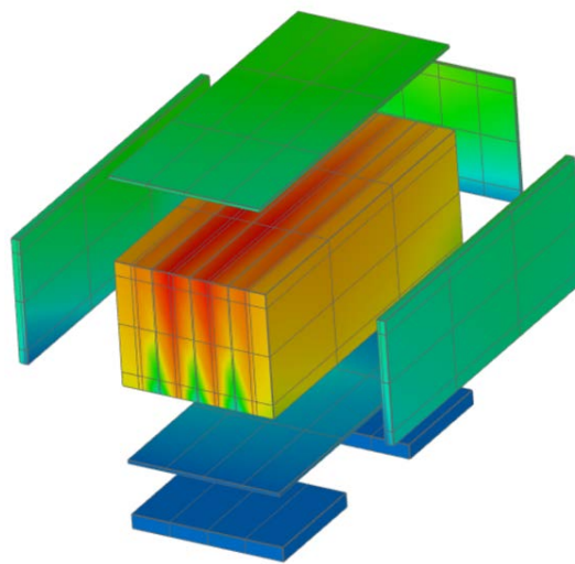
Figure 3. 3D Results – Temperature distribution in Battery Module
