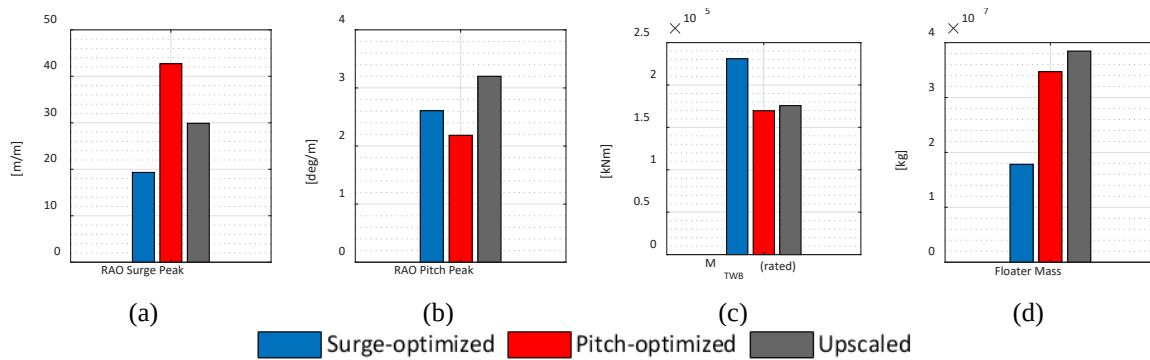
Figure 2. Comparison between the Surge-optimized (blue), the Pitch-optimized (red) and the upscaled (grey) systems: Peak of Surge (a) and Pitch (b) DoFs, Tower-base Bending moment (c) and Floater Mass (d).
