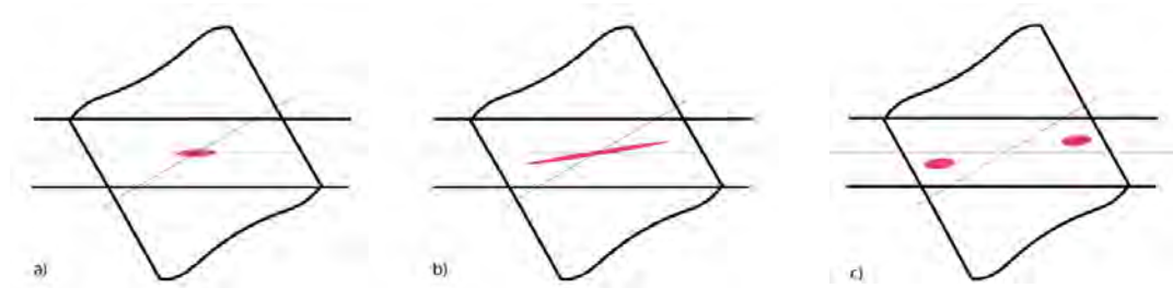
Figure 2. Contact area roller-bar with decreasing angle between roller and bar axes
