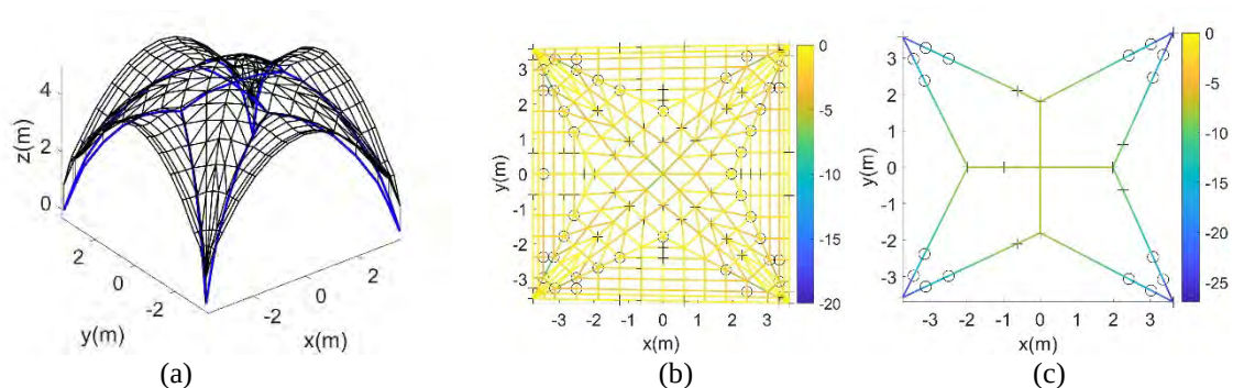
Figure 16 - Two-layer funicular network (with 221 parameters): overall view (a); overlying layer - webbing (b); underlying layer - ribs (element forces are in kN).
