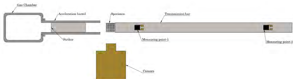
Figure 1. Direct impact Hopkinson bar (DIHB) configuration
