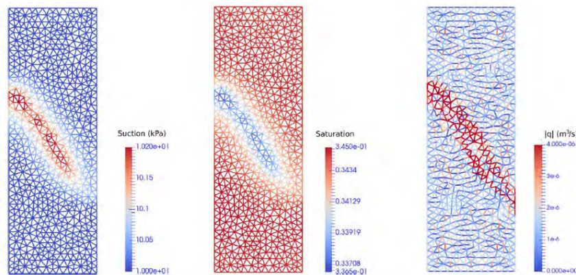
Figure 2. Shear band example, unsaturated sand specimen
