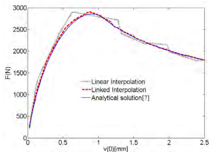
Figure 2. Comparing the performance of linear and linked interpolation for L_e=20\text{mm}
