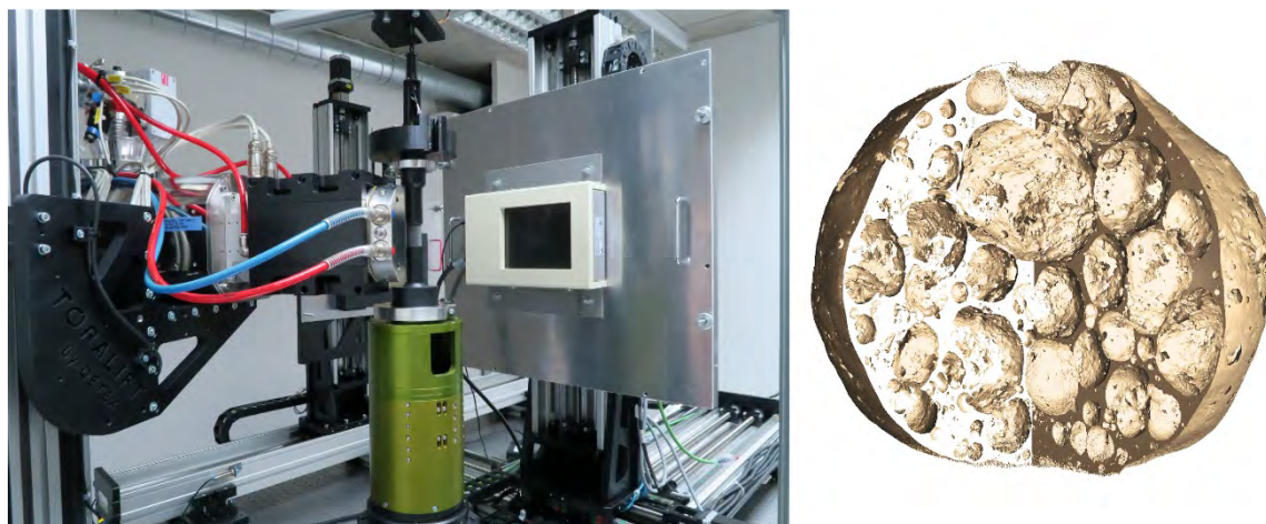
Figure 1. Experimental setup (left), visualization of APM foam element microstructure (right)
