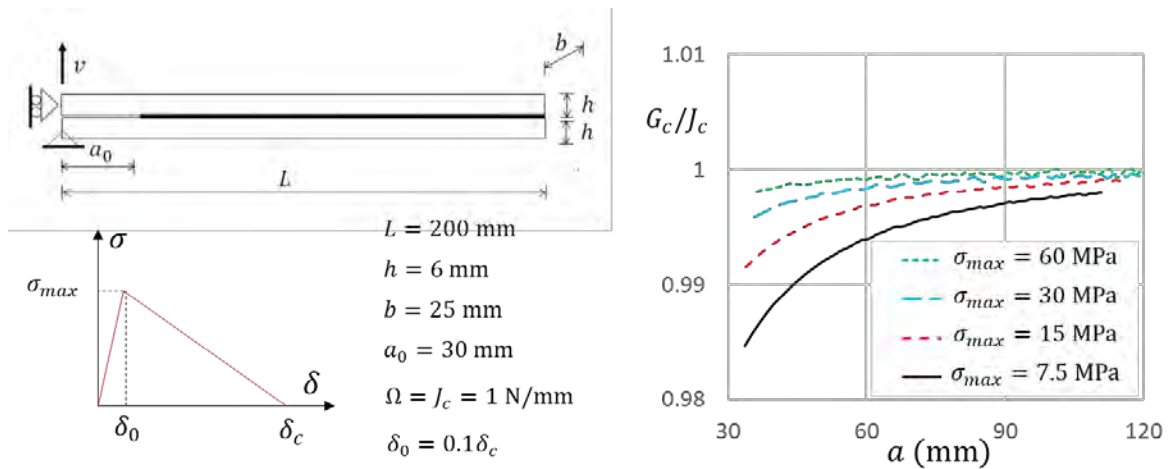
Figure 1. Relation between J_c = \Omega and G_c for numerical simulations of a DCB.
