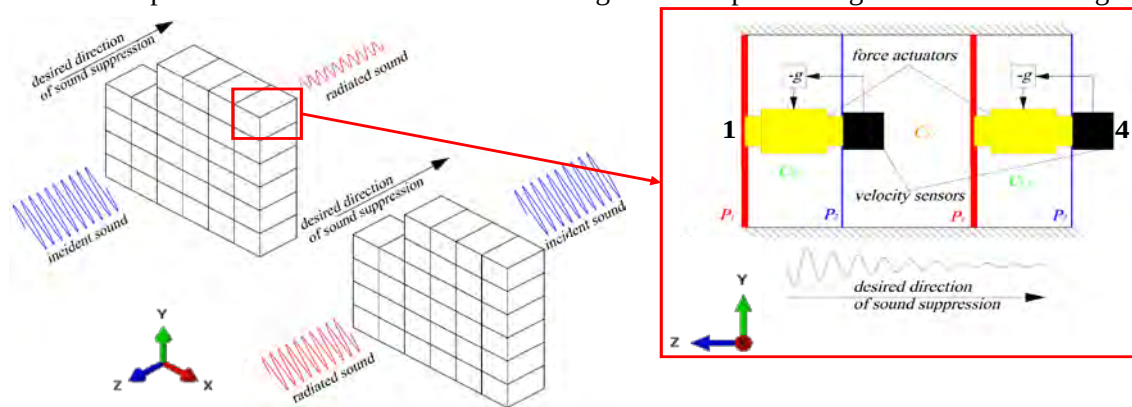
Figure 11 Active metamaterial barrier (left) and single cell concept (right)
