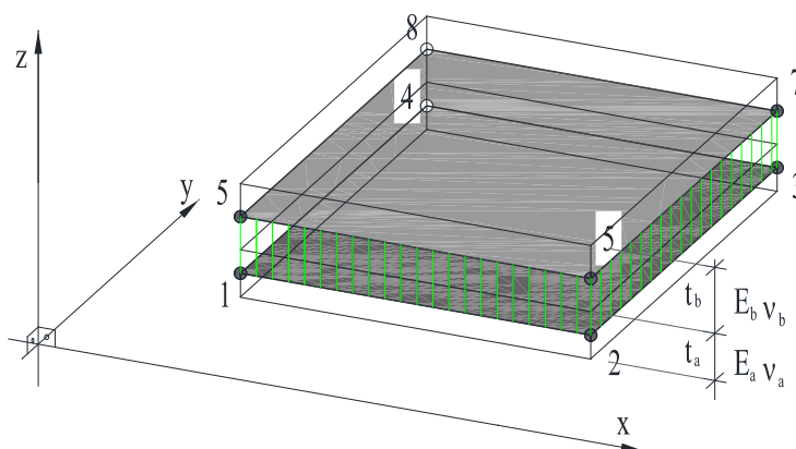
Figure 1. 8-node cohesive element between two layer facet shell elements: 1-2-3-4 and 5-6-7-8
