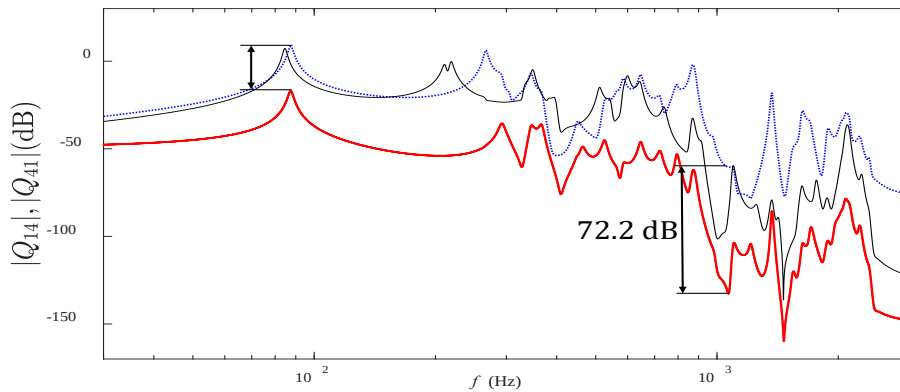
Figure 13 Amplitudes of the characteristic frequency response functions of the activated system Q_{14} and Q_{41} : faint black line – passive system (reference), dotted blue line – Q_{14} , solid red line – Q_{41}
