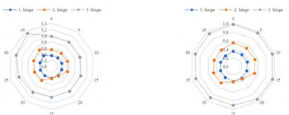
Figure 1. Masonry arch bridge horizontal support displacement vs. square span ratio (left) and skewed span ratio at hinge opening (%) w. r. t. skew angle (°)
