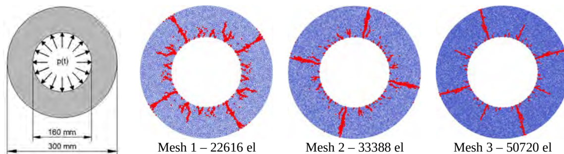
Figure 1. Thick cylinder test
