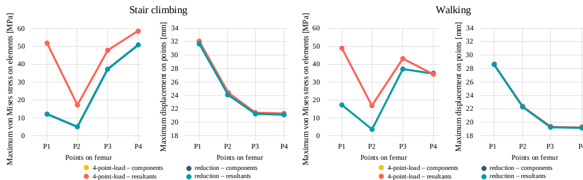
Figure 2. Maximum von Mises stress distribution and displacements for the two load cases
