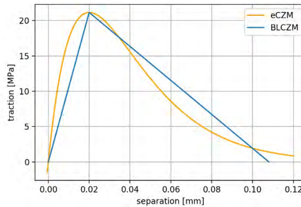
Figure 2. Exponential (eCZM) vs. bi-linear (BLCZM) traction-separation law with equal maximum traction
