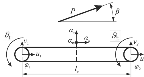
Figure 1. Piezoelectric beam element
