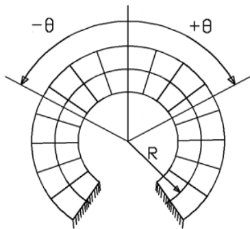
Figure 1. Helical girder [4]
