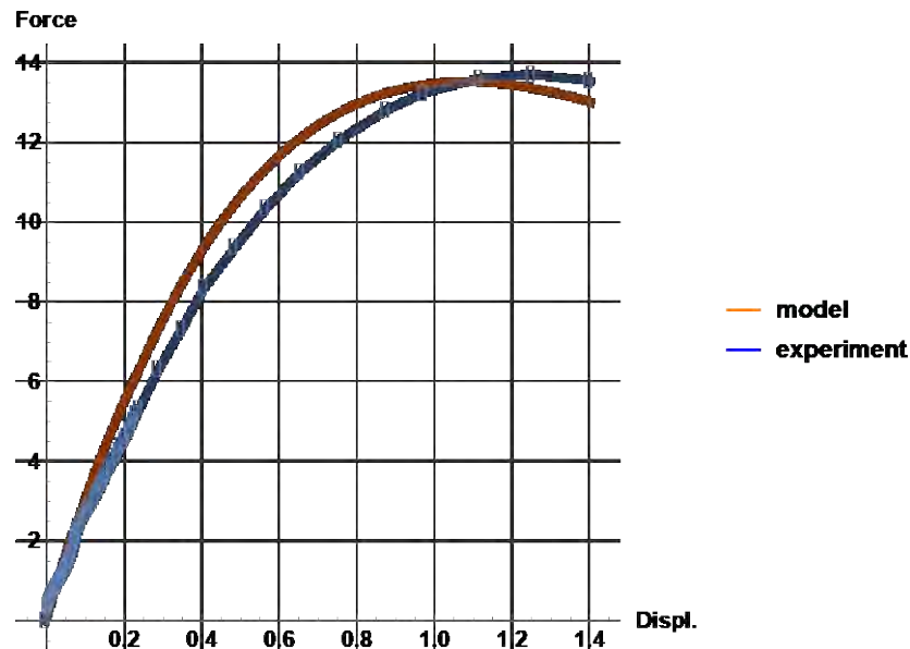
Figure 2. Experimental results, displacement - force diagram
