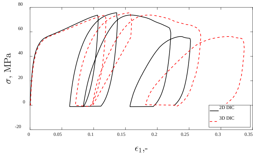
Figure 1. Comparison of the material response obtained from 2D and stereoDIC measurements
