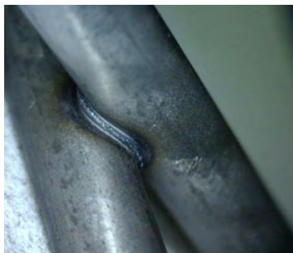
Figure 1 Close up image of the weld taken with the microscope
