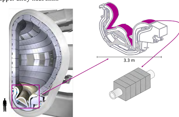
Figure 1. Cross-section of a fusion reactor, with the divertor components highlighted
